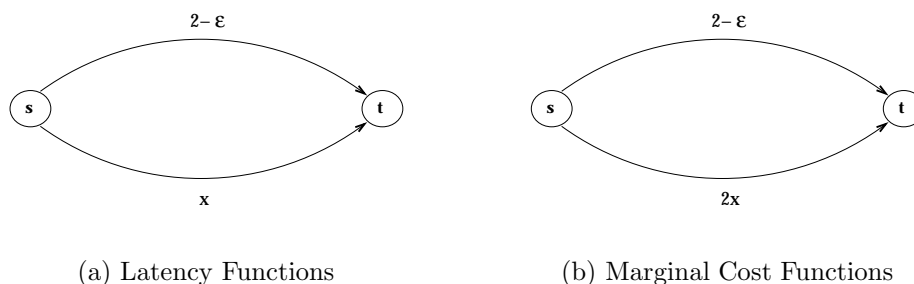
Figure 2.5: The optimal flow may sacrifice some traffic to a path with large latency to minimize the total latency.
