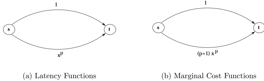
Figure 2.4: A nonlinear variant of Pigou's example
