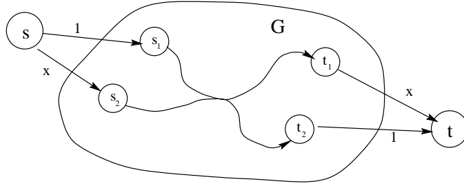
Figure 5.1: Proof of Theorem 5.3.2. In a “no” instance of 2DDP, existence of s_1-t_1 and s_2-t_2 paths implies the existence of an s_2-t_1 path.
