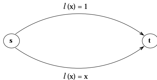
Figure 1.1: Pigou’s example. A latency function \ell(x) describes the delay experienced by drivers on a road as a function of the fraction of overall traffic using that road.
