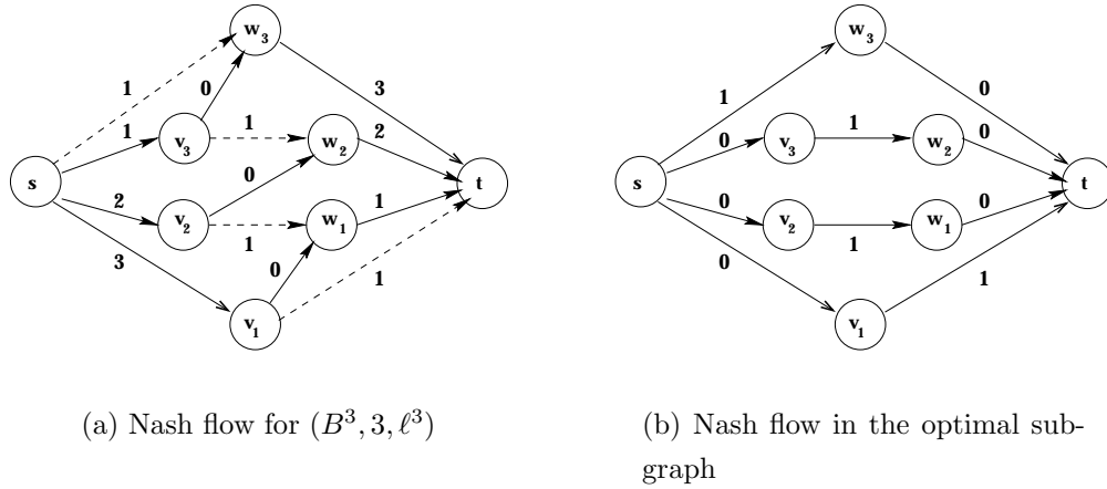
Figure 5.4: Proof of Proposition 5.4.2, when k = 3 . Solid edges carry flow in the flow at Nash equilibrium, dashed edges do not. Edge latencies are with respect to flows at Nash equilibrium.
