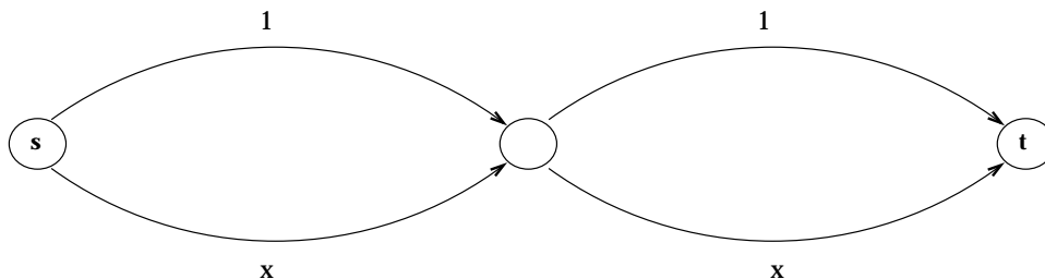
Figure 2.3: The Nash flow may be strictly Pareto-dominated by the optimal flow in the absence of Braess’s Paradox.
