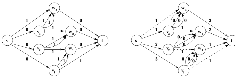
(a) A good Nash flow corresponding to a “yes” instance of PARTITION, with m = 2
