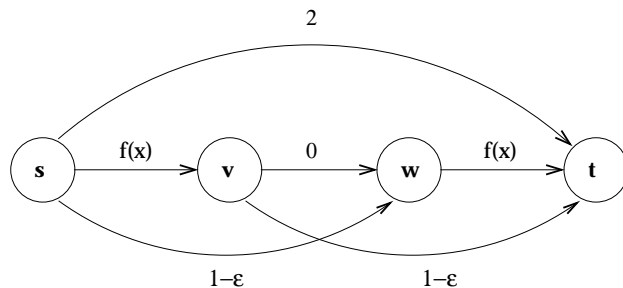
Figure B.1: Theorem 4.1.3 is sharp
