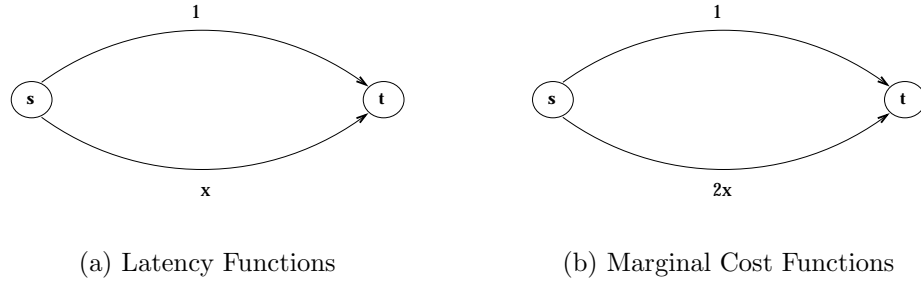
Figure 2.1: Pigou's example revisited
