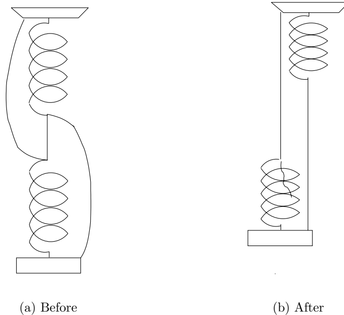
Figure 1.3: Strings and springs. Severing a taut string results in the rise of a heavy weight.
