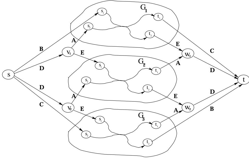
Figure 5.6: Proof of Theorem 5.5.6. Construction of (G', k, \ell) when k = 3 . Edges are labeled with their edge type.
