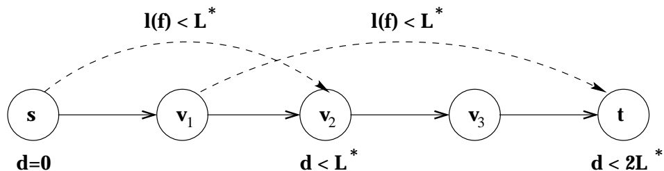
Figure 5.2: Proof of Theorem 5.4.1. If f is the flow sending one unit of flow on the four-hop path and f^* is the flow sending half a unit of flow on each of the other two paths, then the dashed edges are light.
