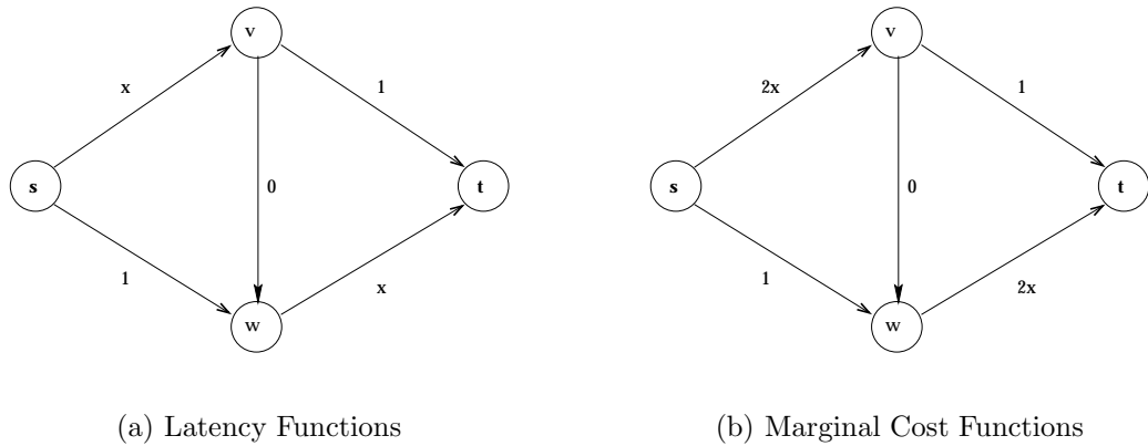
Figure 2.2: Braess's Paradox revisited
