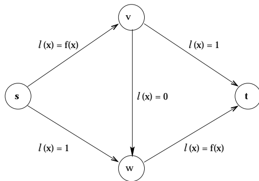
Figure B.2: A bad example for Stackelberg routing
