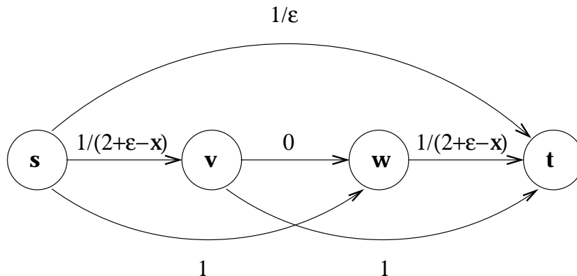
Figure 4.1: A Bad Example for Unsplittable Flow
